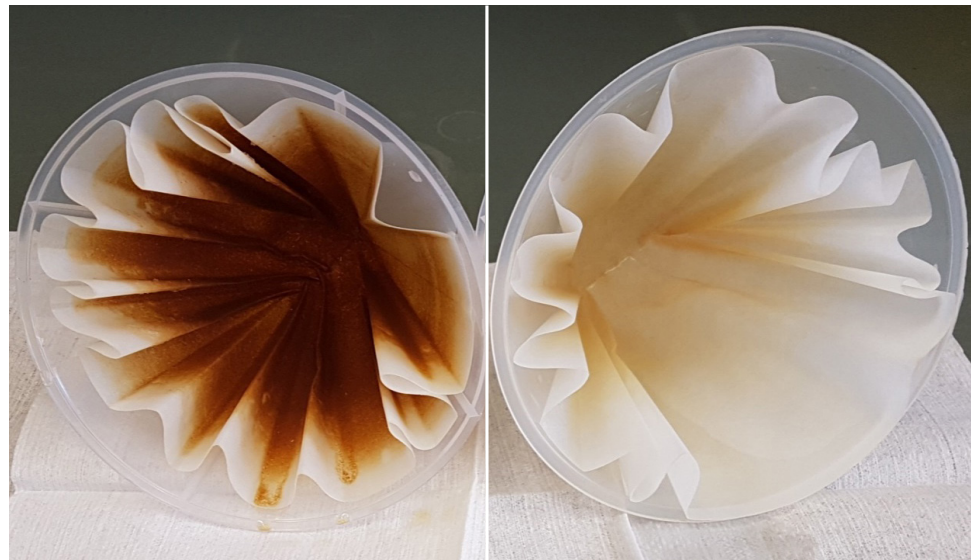
Figure 1: Low Pd precipitation / low sludge formation (11 m 2 /L throughput). Left: Standard activation, right: Neoganth® E Activator System
